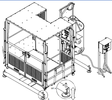
BASE – CABINA
